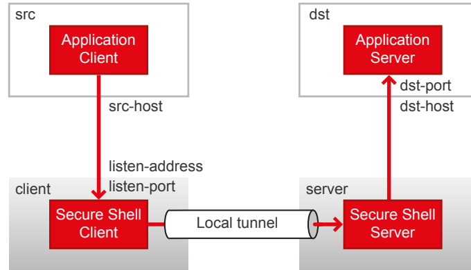
Figure 9.1. Local tunneling terminology
