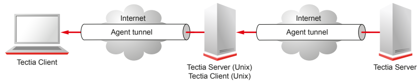
Figure 7.6. Agent forwarding
